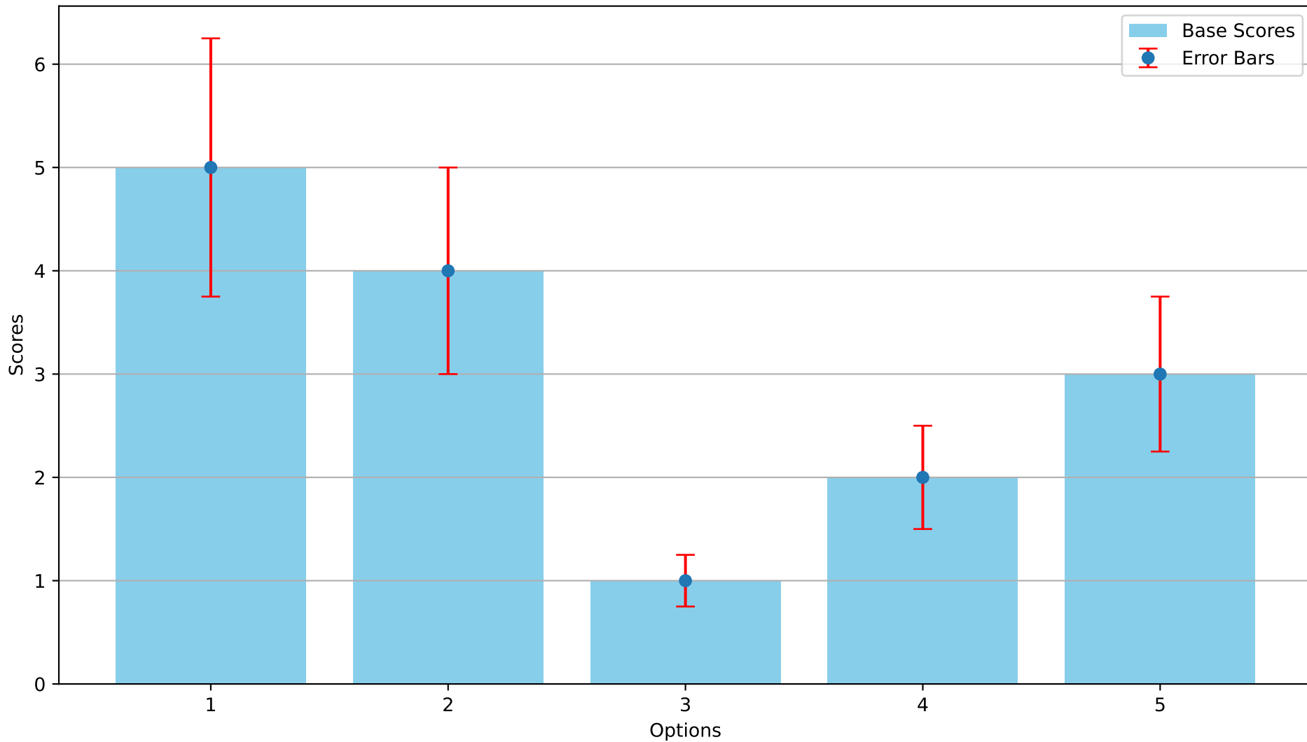
Combined Result Sensitivity Analysis for Ease of Disassembly
